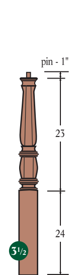
O 4210 - 48" octagon - oak
