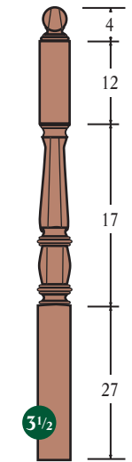
O 4203 - 60 octagon - oak
