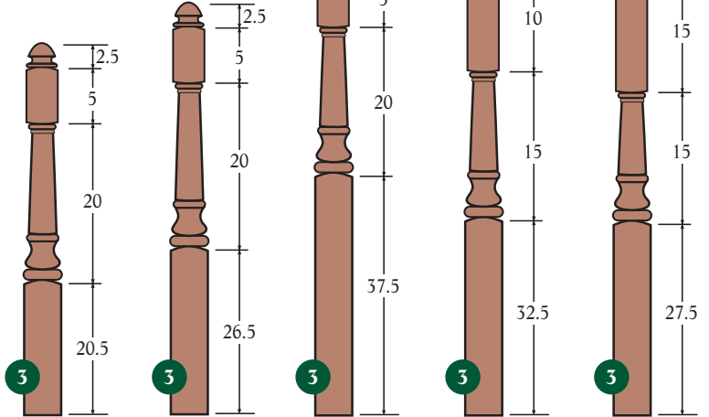
A4180-48/52 A4181-54 A4182-60,72 A4183-60 A4184-60 oak, poplar, maple square bottom oak, poplar, maple square bottom oak, poplar, maple square bottom oak, poplar, maple square bottom oak, poplar, maple square bottom
