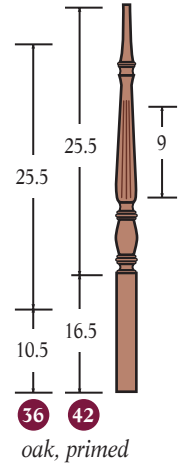
F 5315 R-1 3/4" square bottom
