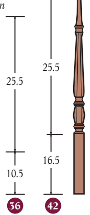
O 5315 R - 1 3/4" square bottom octagon
