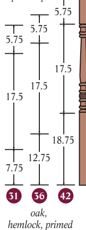
A 5005 S - 1 3/4" square bottom square top
