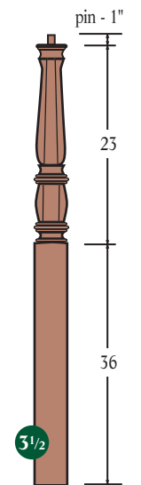
O 4215 - 60" octagon - oak
