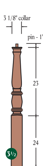
A 4210 - 48" oak, maple, cherry, mahogany
