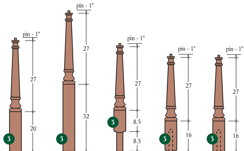
A4010-48 A4015-60/72 R4012-45 R4016-44 S4016-44 oak/poplar/maple oak/poplar/maple oak round bottom oak/maple round bottom, pin included oak/maple square bottom pin included
