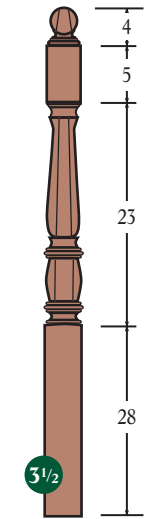
O 4201 - 60 octagon - oak
