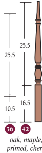
A 5315 R-1 3/4" square bottom
