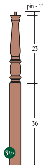
A 4215 - 60" oak, maple, cherry, mahogany
