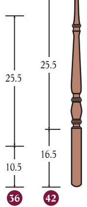
R 5315 R - 1 3/4" round bottom
