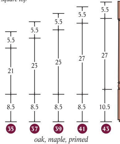
A 5070 S - 1 1/4" square top
