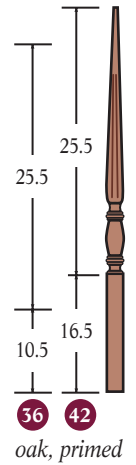
F 5311 R-1 1/4" square bottom
