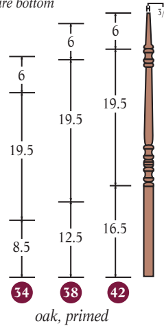
A 5200 R - 1 1/4" square bottom
