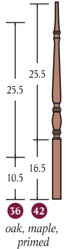
A 5301 R-1 1/4" square bottom
